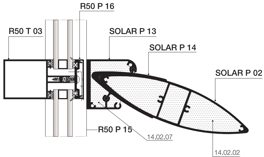
KESİT SECTION
