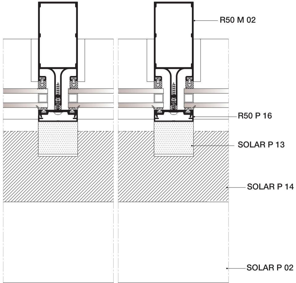
PLAN PLAN
